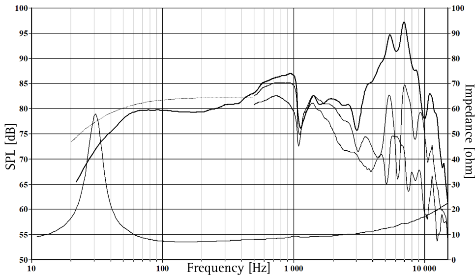
The frequency responses above show measured free field sound pressure in 0, 30, and 60 degrees angle using a 22L closed box. Input 2.83 VRMS, microphone distance 0.5m, normalized to SPL 1m. The dotted line is a calculated response in infinite baffle based on the parameters given for this specific driver. The impedance is measured in free air without baffle using a 2V sine signal.
